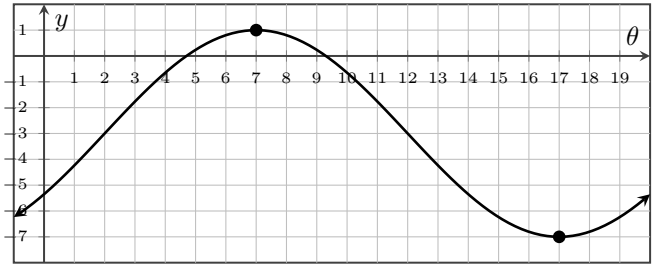
Figure 6.6: A Graph of y = H(\theta)
